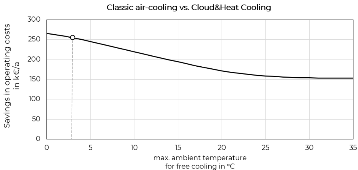
Illustration 6: Potential savings in operating costs, in relation to the maximum ambient temperature 16 at which free cooling is possible - classic air cooling vs. Cloud&Heat Cooling
