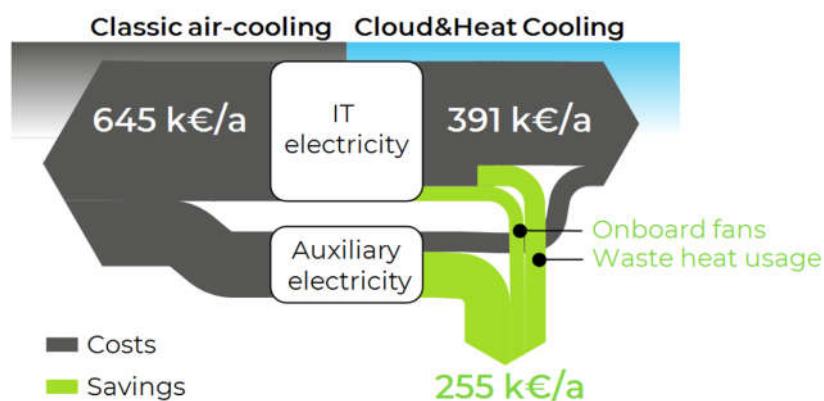
Illustration 5: Cost flow diagram - standard air-cooling vs. Cloud & Heat Cooling
