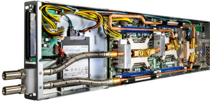
Illustration 1: 100 % water-cooled Blade from Megware
