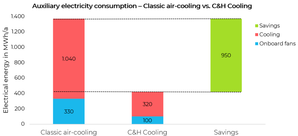
Illustration 4: Auxiliary electricity consumption – classic air-cooling vs. Cloud&Heat Cooling
