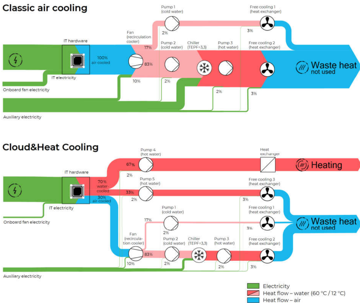
Illustration 3: Energy flow diagram - classic air cooling vs. Cloud&Heat Cooling
